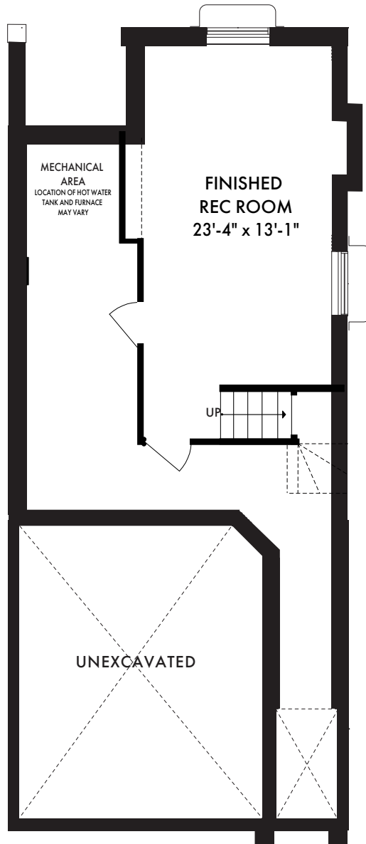
STANDARD BASEMENT
