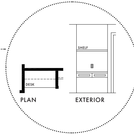
SECOND FLOOR OPT. BEDROOM DESK
