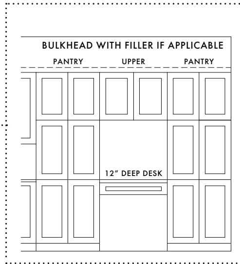
GROUND FLOOR OPT. PANTRY EXTENSIONS
