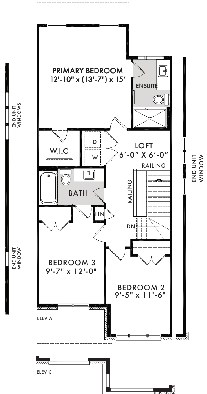
SECOND FLOOR
