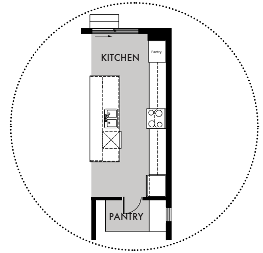
GROUND FLOOR OPT. CHEF'S KITCHEN LAYOUT
