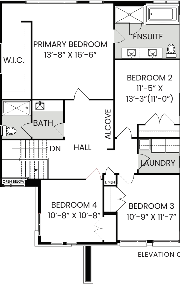
STANDARD SECOND FLOOR
