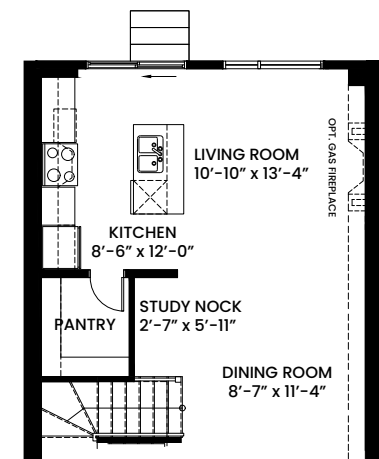
GROUND FLOOR PLAN OPT. KITCHEN WITH PANTRY B
