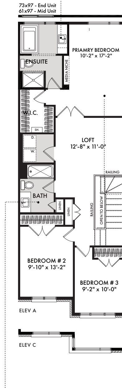
SECOND FLOOR
