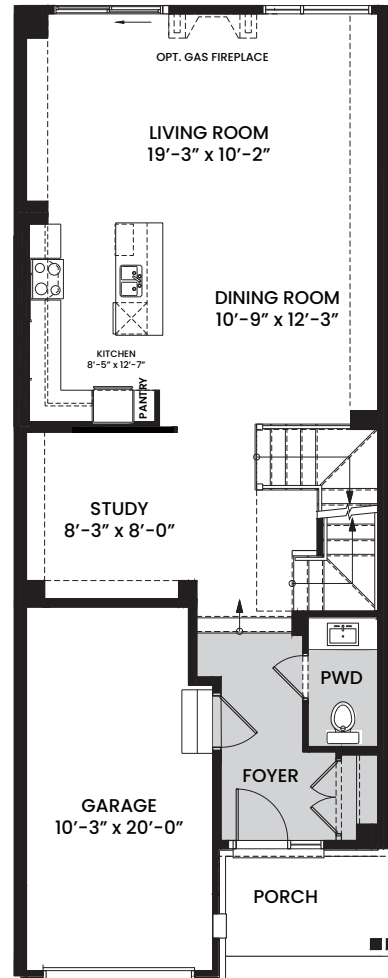
GROUND FLOOR PLAN OPT. KITCHEN
