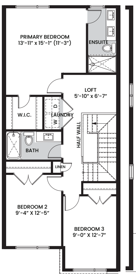
STANDARD SECOND FLOOR
