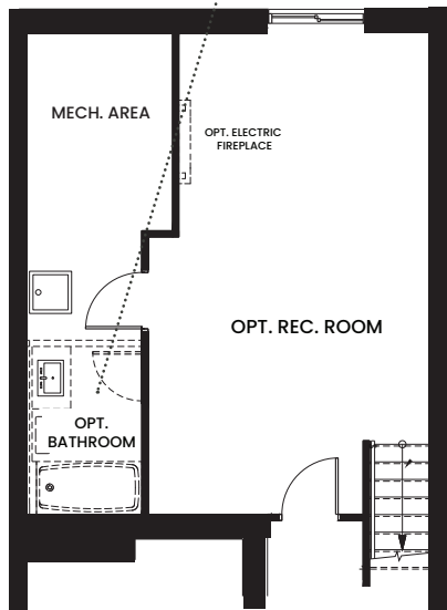
BASEMENT FLOOR PLAN OPT. FINISHED REC. ROOM 279 SQ. FT.
