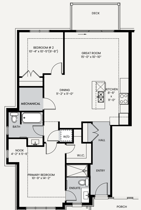
MAYFAIR SPECIAL STREET END UNIT - 1080 SQ FT
