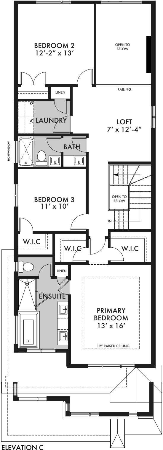
STANDARD SECOND FLOOR **INCLUDES 125 SQ FT OF OPEN SPACE
