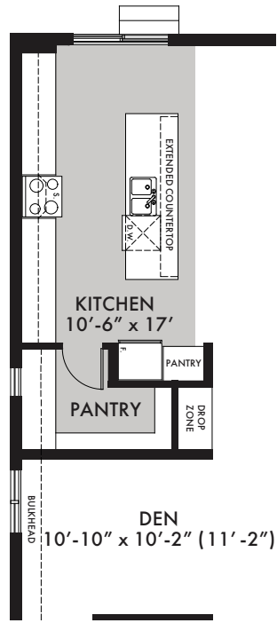
GROUND FLOOR OPT. KITCHEN
