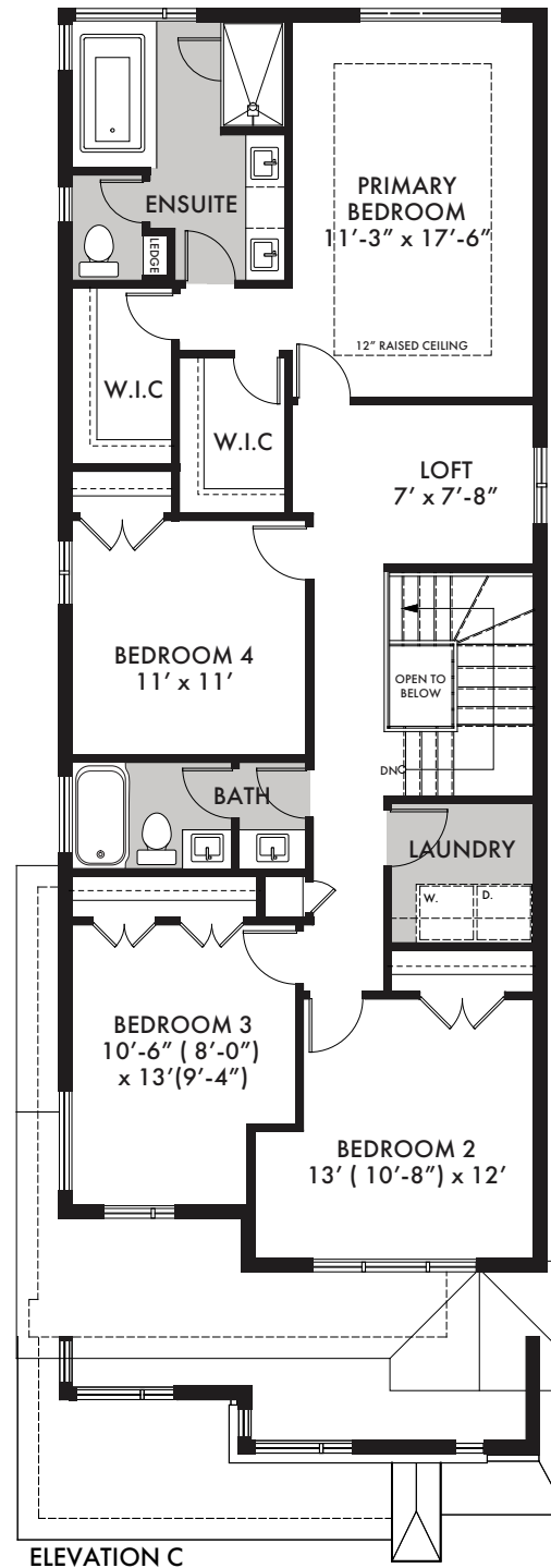
SECOND FLOOR OPT. ALTERNATE 4 BEDROOM WITH LOFT
