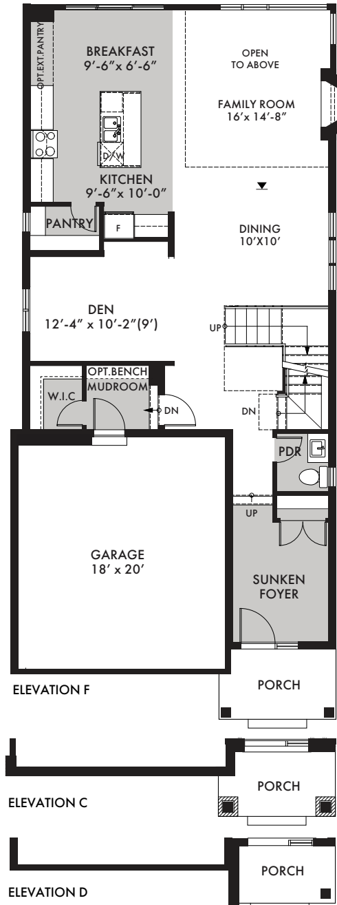
STANDARD GROUND FLOOR
