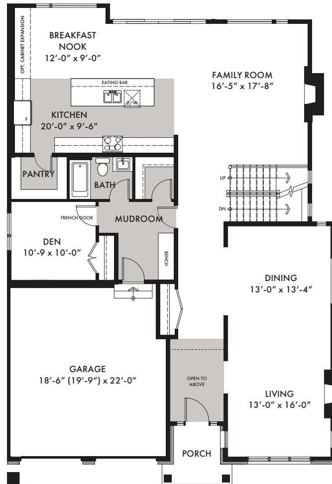
ELEVATION F
