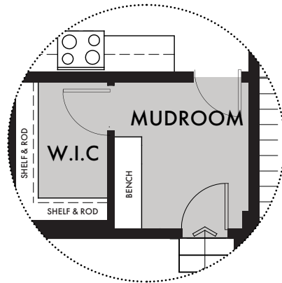
GROUND FLOOR OPT. MUDROOM AND W.I.C.
