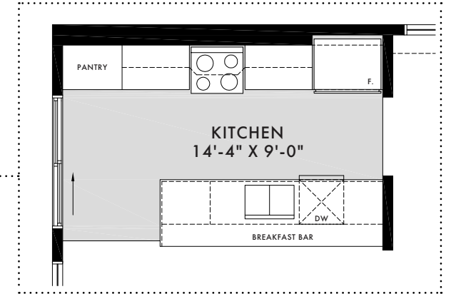
GROUND FLOOR OPT. CHEF'S KITCHEN
