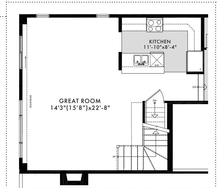
GROUND FLOOR OPT. CHEF'S KITCHEN
