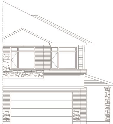
ELEVATION C
