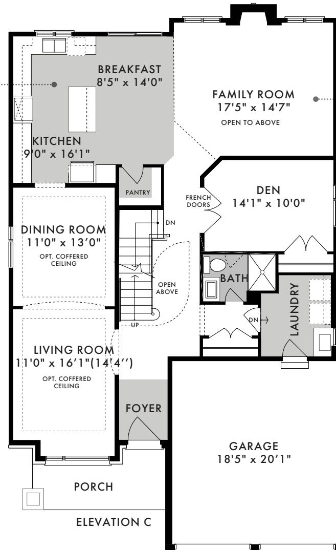
STANDARD GROUND FLOOR
