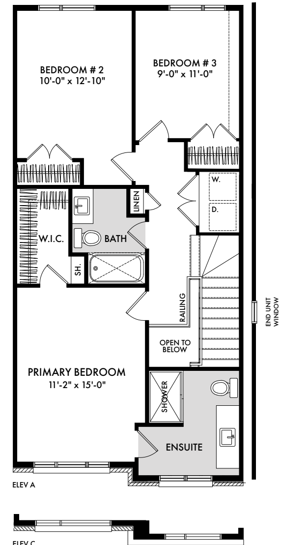
SECOND FLOOR
