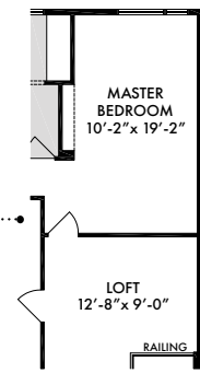
SECOND FLOOR OPT. PRIMARY BEDROOM WITH REDUCED LOFT
