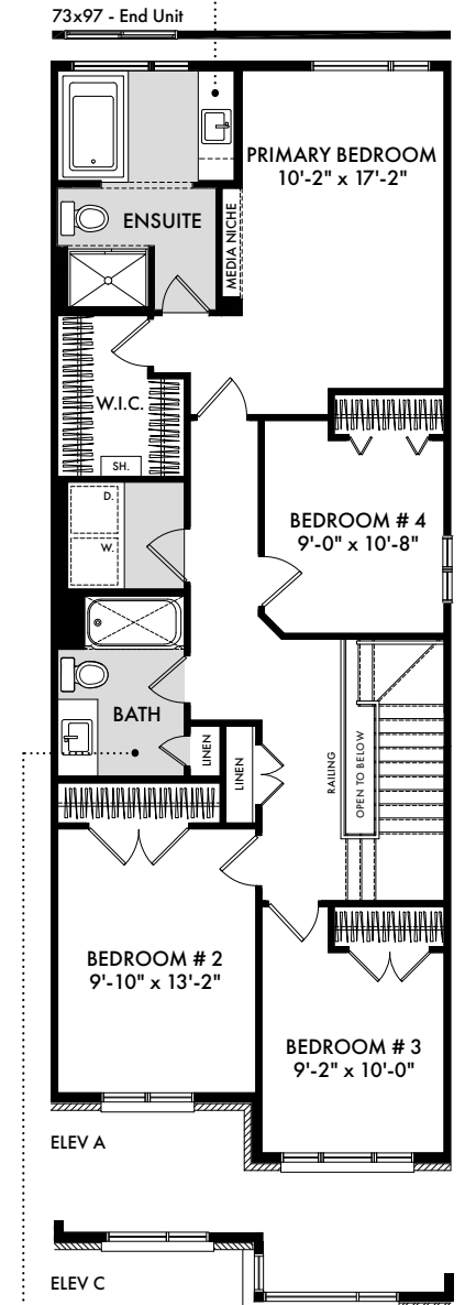
SECOND FLOOR OPT. ENSUITE WITH EXTENDED W.I.C.
