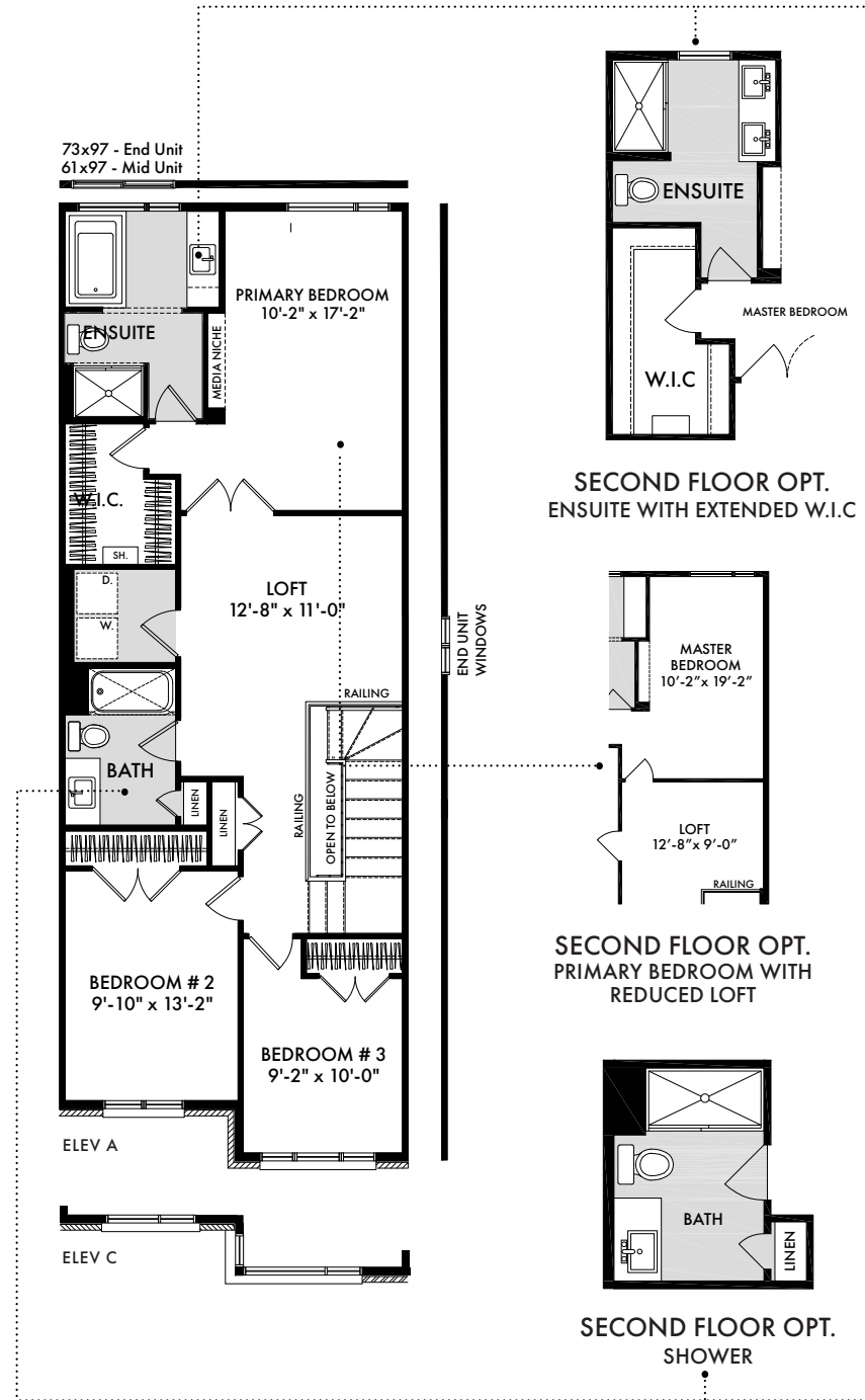
SECOND FLOOR
