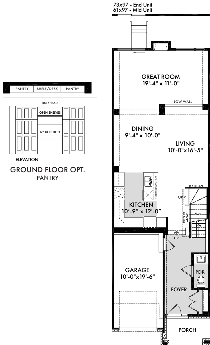
GROUND FLOOR
