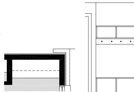
GROUND FLOOR OPTION FOYER BENCH
