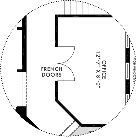
GROUND FLOOR OPTION OFFICE/DEN
