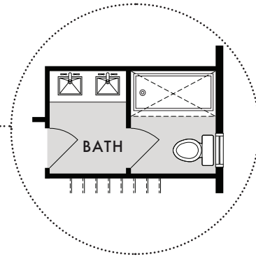
SECOND FLOOR OPTION DOUBLE SINKS
