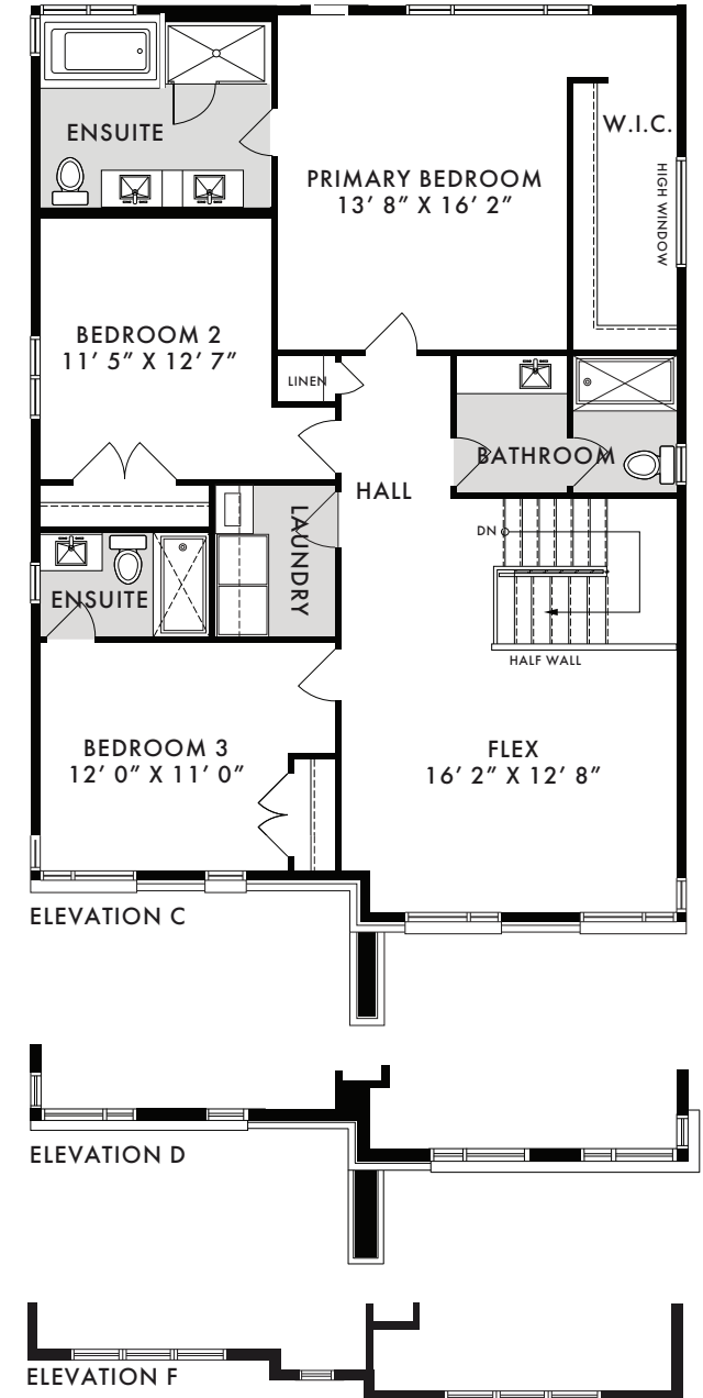
STANDARD SECOND FLOOR
