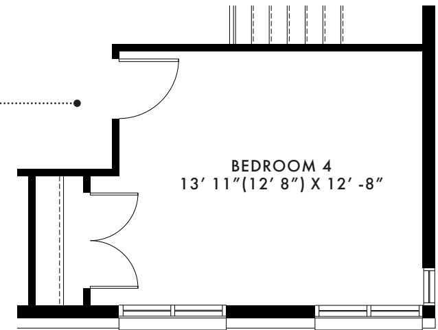
SECOND FLOOR OPTION 4 BEDROOM
