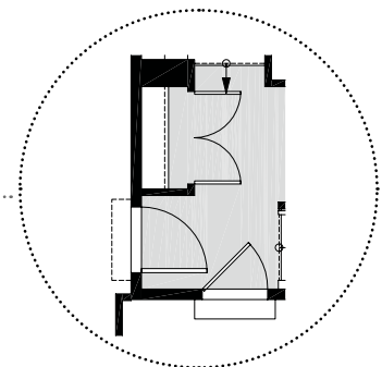
GROUND FLOOR OPTION MUD ROOM DOOR
