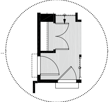
GROUND FLOOR OPTION MUD ROOM DOOR
