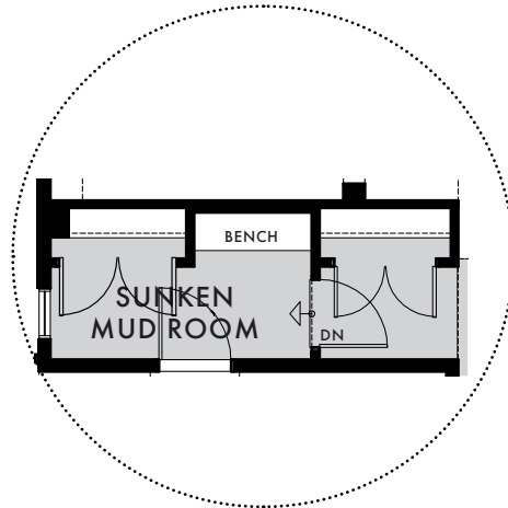
GROUND FLOOR OPTION MUD ROOM BENCH
