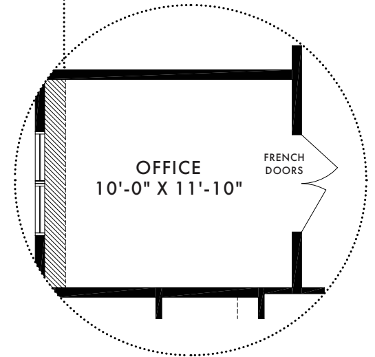
GROUND FLOOR OPTION OFFICE
