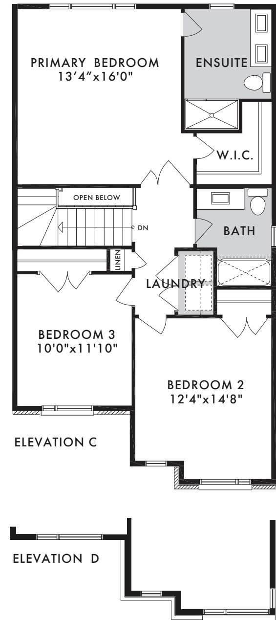
STANDARD SECOND FLOOR
