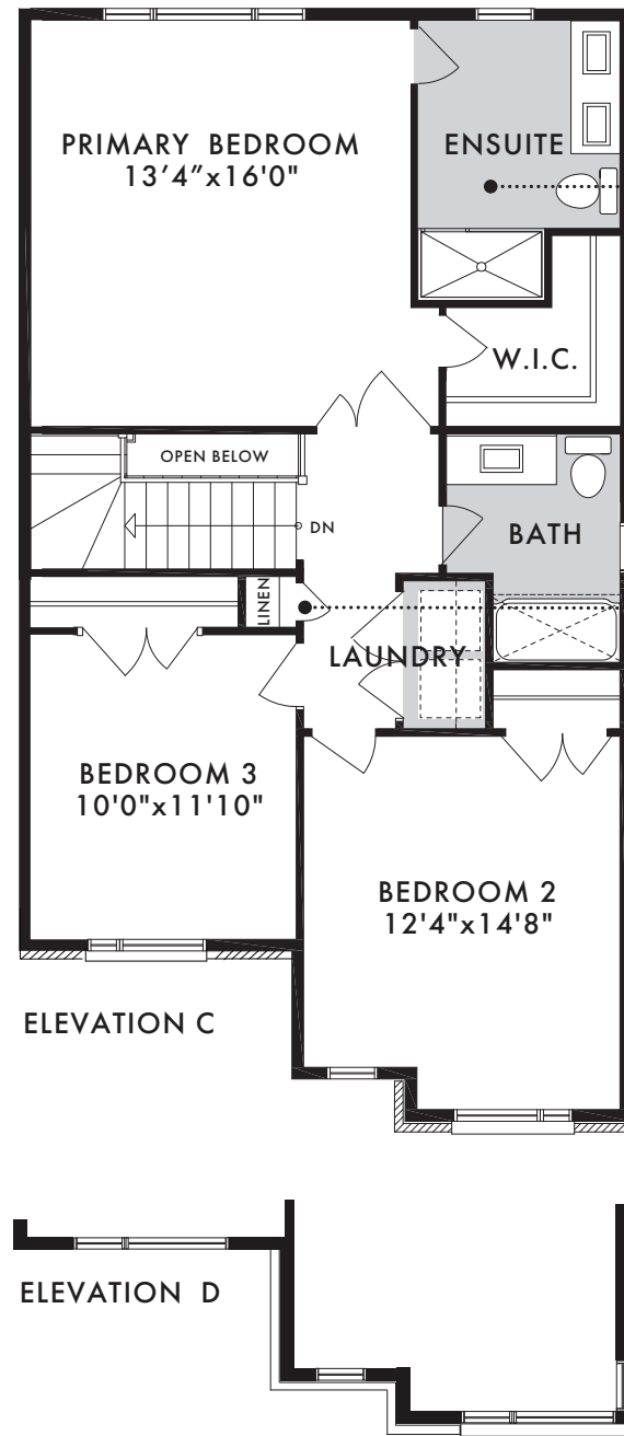
SECOND FLOOR OPT.
